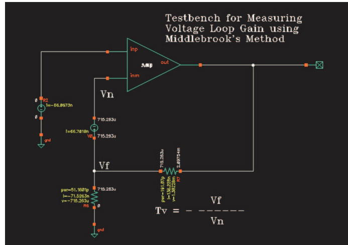
Figure 1: Middle Brook Voltage Loop Gain Testbench
