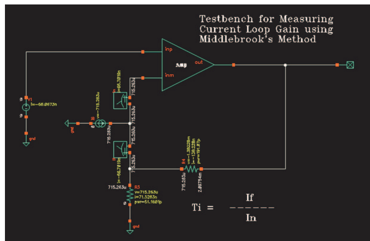
Figure 2: Middlebrook Current Mode Loop Gain Testbench
