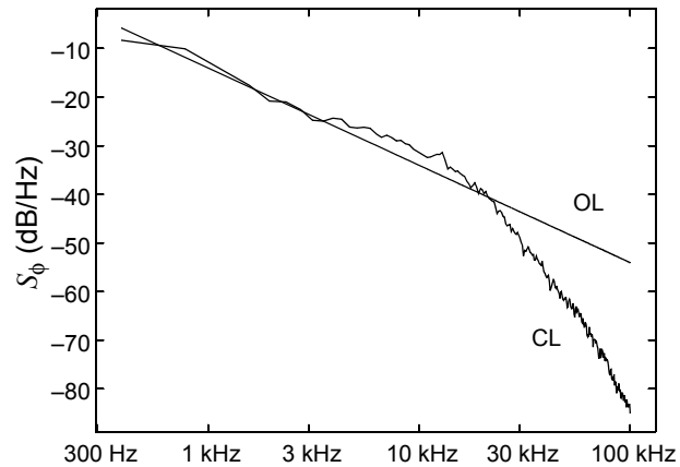
FIGURE 17 Noise of the closed-loop PLL at the output of the VCO when only the reference oscillator exhibits jitter (CL) versus the noise of the reference oscillator mapped up to the VCO frequency when operated open loop (OL).
